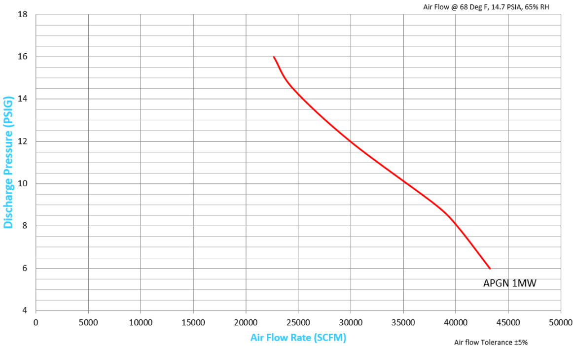
PERFORMANCE CURVE APGN 1.1MW
